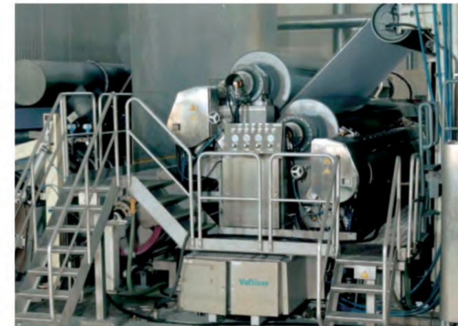
Sizing Machine
